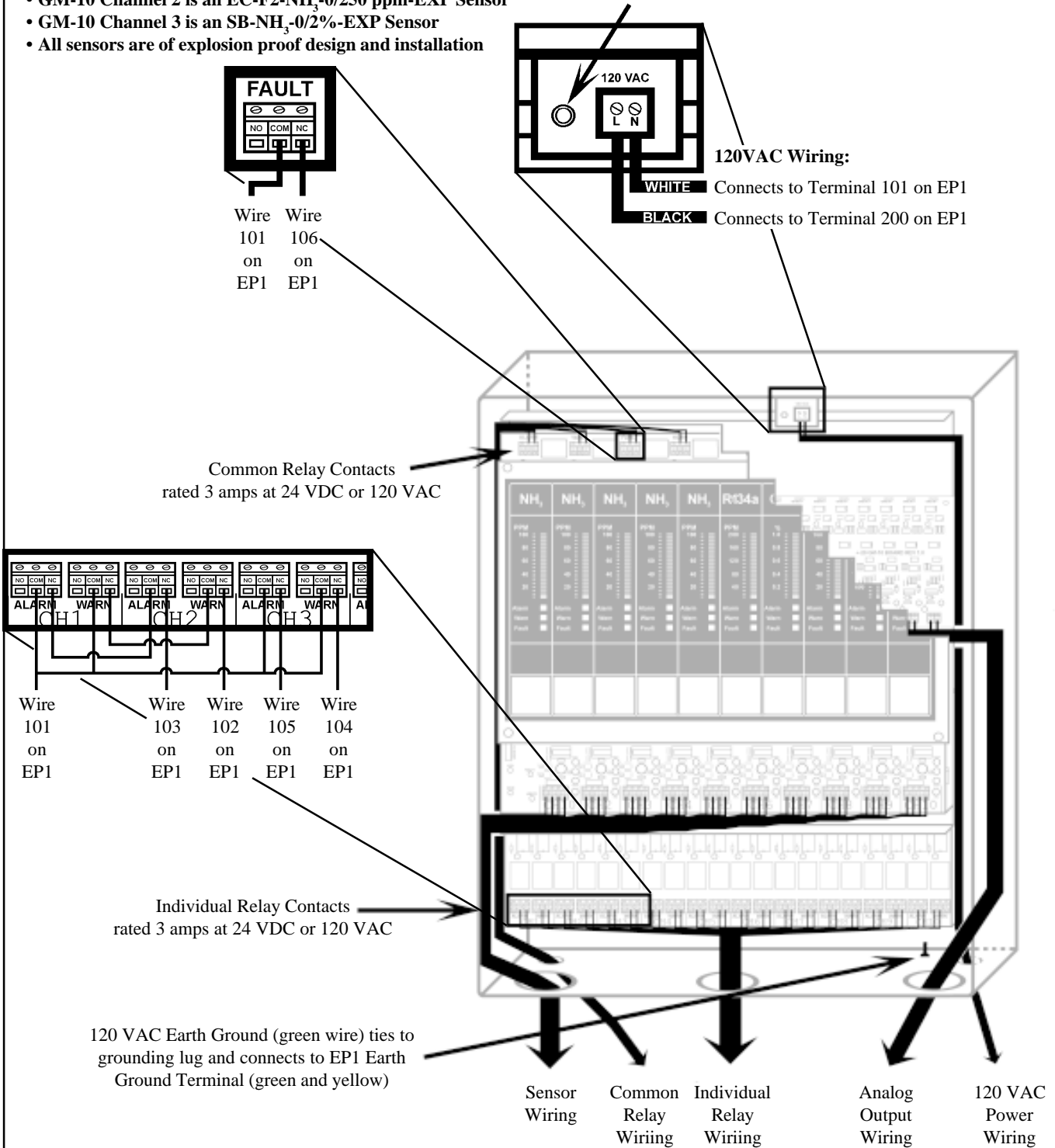
Figure 1: Wiring Diagram for Wiring the GM-10 to the EP1 Shutdown Panel
