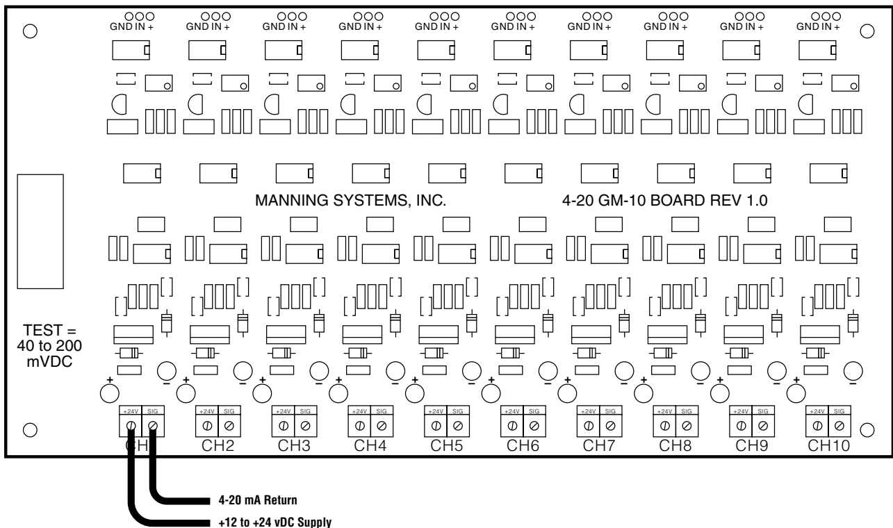
Figure 1: Wiring Diagram for the GM-10 Analog Output Board
