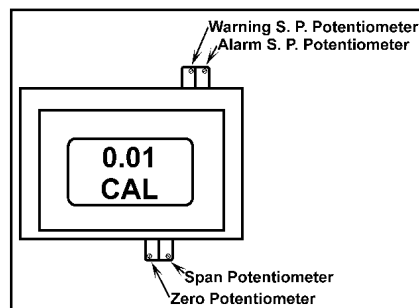
Figure 2: Potentiometers
