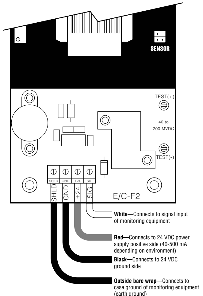
Figure 2: Wiring Diagram for the Manning EC-F2 Sensor
