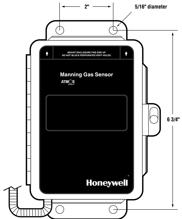
Figure 1: Mounting Dimensions
