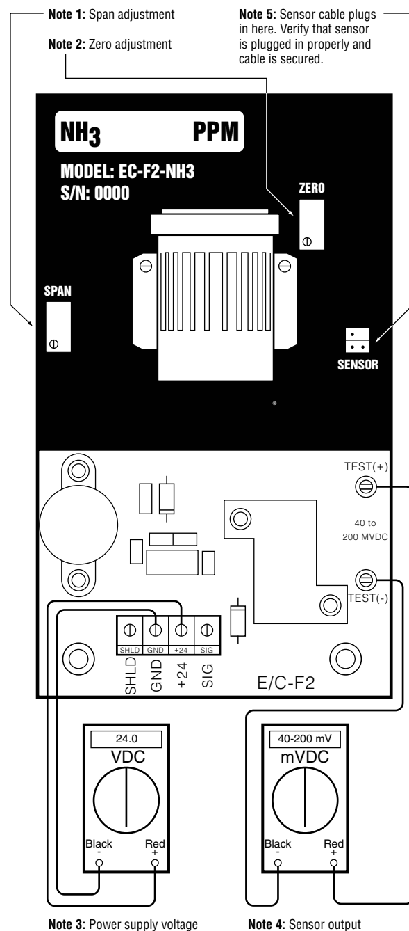
Figure 3: Checking sensor output, power supply voltage, and zero and span adjustments
